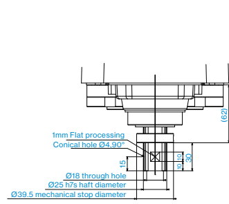
Detail of "A" (Calibration point position of Joints #3 and #4)
