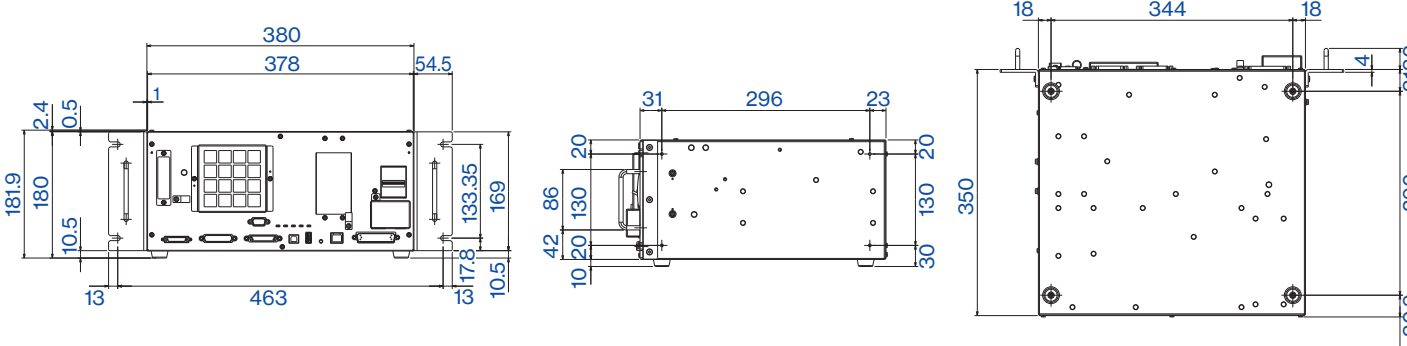
Outer Dimensions [Unit: mm]
