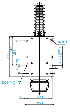
Reference through hole (View from bottom of the base)
